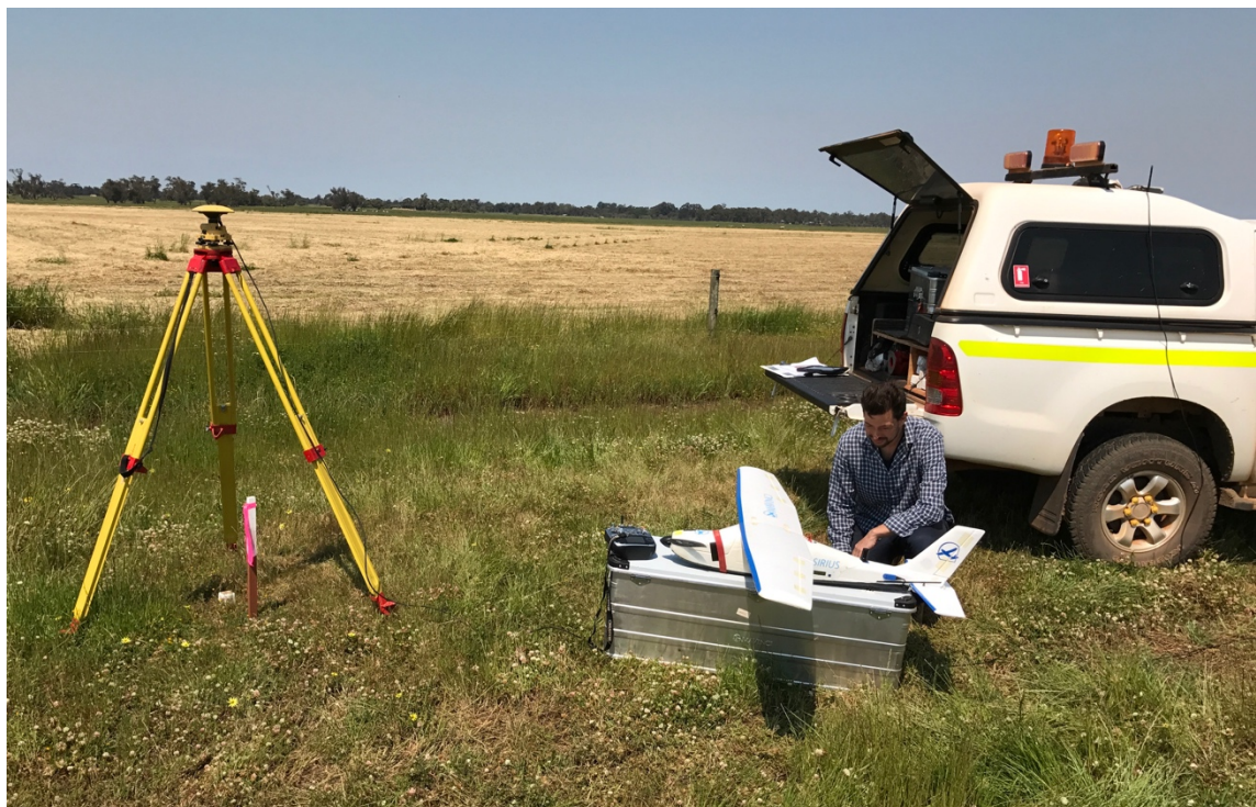
Figure 1: Sirius MAVinci Pro UAV at SER's Ambergate Mineral Sands Project
